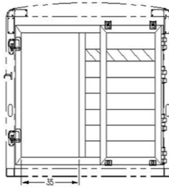
PASS-THROUGH WIDTH STANDARD SLIDING REAR GATE SHOWN WITH ROLLER GATE OPEN
