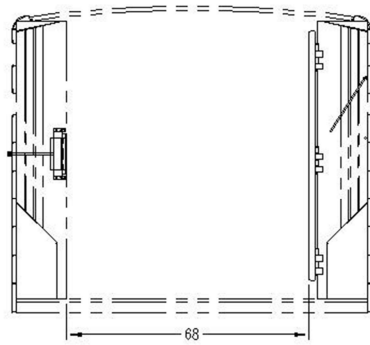
PASS-THROUGH WIDTH W/ 8K AXLES SHOWN WITH CENTER GATE OPEN
