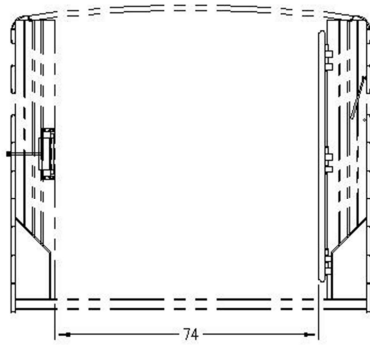
PASS-THROUGH WIDTH W/ 6K, 7K OR 7.2K AXLES SHOWN WITH CENTER GATE OPEN
