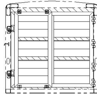
7'4" TALL, SLOTTED ROLLER GATE REAR OPENING - 82W X 84T
