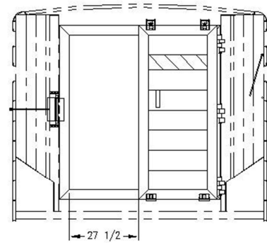
PASS-THROUGH WIDTH W/ 10K AXLES SHOWN WITH CENTER GATE OPEN
