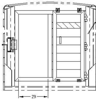
PASS-THROUGH WIDTH W/ 8K AXLES SHOWN WITH ROLLER DOOR OPEN
