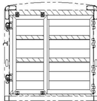
6'8" TALL, SLOTTED ROLLER GATE REAR OPENING - 90 1/2" X 76"
