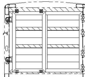
6'8" TALL, SLOTTED ROLLER GATE REAR OPENING - 82W X 76T
