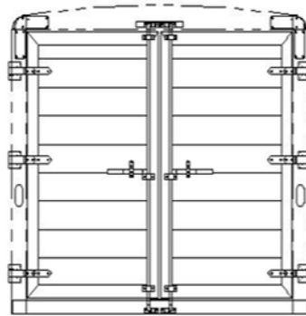
6'8" TALL DOUBLE DOOR REAR OPENING - 88 7/8" X 75" CAM LATCH WITH LAY-FLAT HINGES
