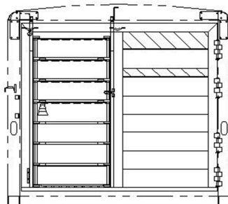
6'8" TALL, HALF ROLL-UP, 32 1/4" OPENING WIDTH REAR OPENING - 82W X 76T
