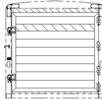
7'4" TALL, SOLID GATE REAR OPENING - 82W X 84T
