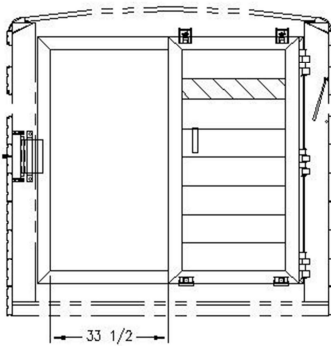
PASS-THROUGH WIDTH W/ 6K, 7K OR 7.2K AXLES SHOWN WITH ROLLER DOOR OPEN
