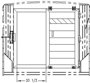
PASS-THROUGH WIDTH W/ 6K, 7K OR 7.2K AXLES SHOWN WITH CENTER GATE OPEN
