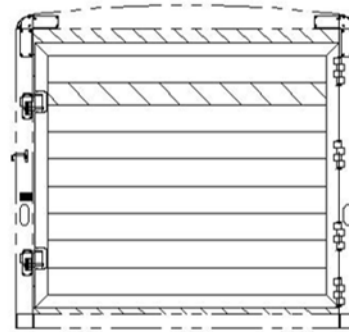
7'4" TALL SOLID GATE REAR OPENING - 90 1/2" W X 84" T
