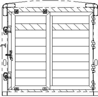
7'4" TALL, STANDARD LIVESTOCK SLIDER REAR OPENING - 82W X 84T
