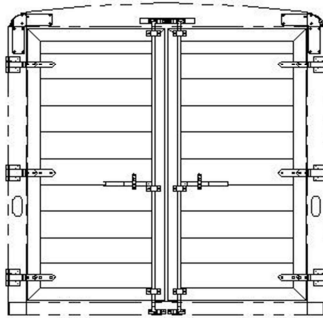
7'4" TALL, DOUBLE DOOR REAR OPENING - 88 7/8W X 83T CAM LATCH WITH LAY-FLAT HINGES
