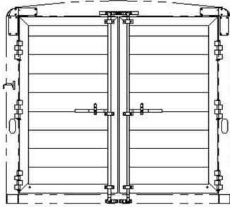
6'8" TALL, DOUBLE DOORS REAR OPENING - 88 7/8" X 75T CAM LATCH WITH STANDARD HINGES
