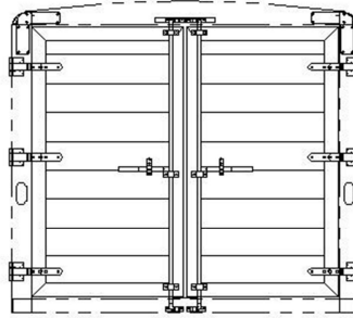
6'8" TALL, DOUBLE DOOR REAR OPENING - 88 7/8" X 75T CAM LATCH WITH LAY-FLAT HINGES
