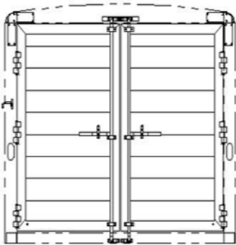
6'8" TALL DOUBLE DOORS REAR OPENING - 88 7/8" X 75" CAM LATCH WITH STANDARD HINGES
