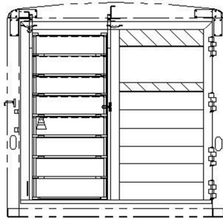
7'4" TALL, HALF ROLL-UP, 32 1/4" OPENING WIDTH REAR OPENING - 82W X 84T
