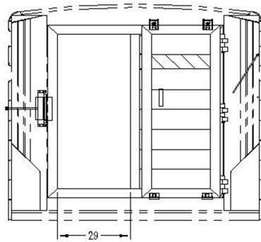
PASS-THROUGH WIDTH W/ 8K AXLES SHOWN WITH CENTER GATE OPEN
