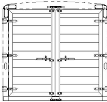
7'4" TALL DOUBLE DOOR REAR OPENING - 88 7/8" W X 83" T CAM LATCH WITH LAY-FLAT HINGES
