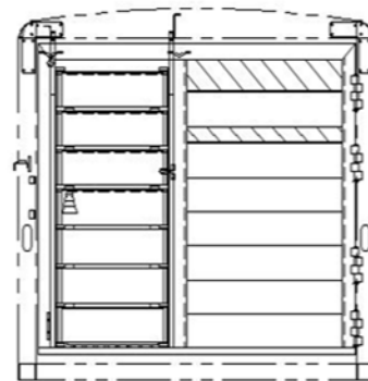
6'8" TALL, HALF ROLL-UP, 32 1/4" OPENING WIDTH REAR OPENING - 90 1/2" X 76"
