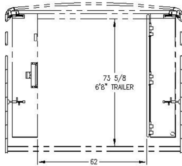
PASS-THROUGH DIMENSIONS ADJUSTABLE POSITION CENTER GATE
