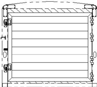
6'8" TALL, ENCLOSED SOLID GATE REAR OPENING - 82W X 76T
