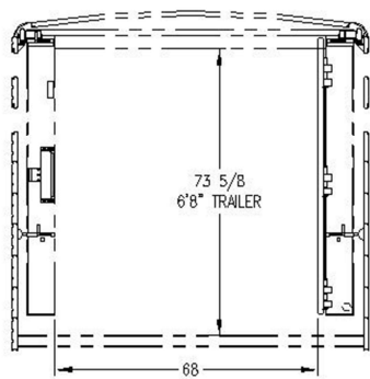
PASS-THROUGH DIMENSIONS ADJUSTABLE POSITION CENTER GATE
