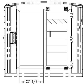
PASS-THROUGH WIDTH W/ 10K AXLES SHOWN WITH ROLLER DOOR OPEN
