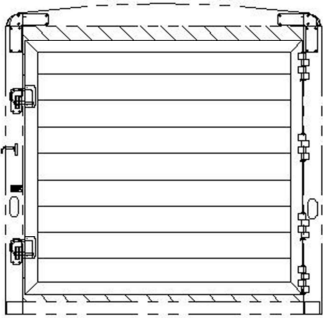
7'4" TALL, ENCLOSED SOLID GATE REAR OPENING - 82W X 84T
