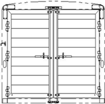
6'8" TALL DOUBLE DOORS REAR OPENING - 88 7/8" X 75" CAM LATCH WITH STANDARD HINGES
