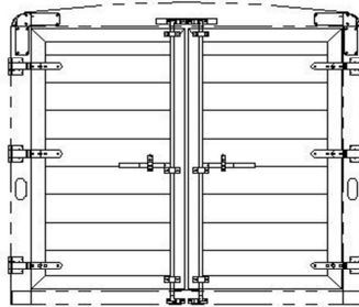
6'8" TALL, DOUBLE DOOR REAR OPENING - 88 7/8W X 75T CAM LATCH WITH LAY-FLAT HINGES
