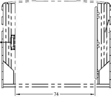
PASS-THROUGH WIDTH W/ 6K, 7K OR 7.2K AXLES SHOWN WITH CENTER GATE OPEN
