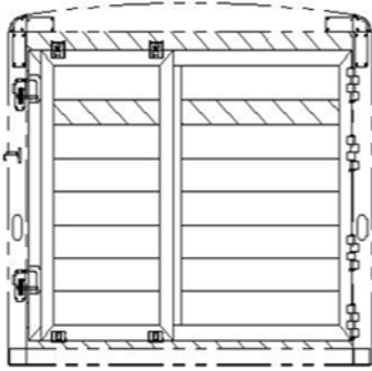
6'8" TALL, STANDARD LIVESTOCK SLIDER REAR OPENING - 90 1/2" X 76"
