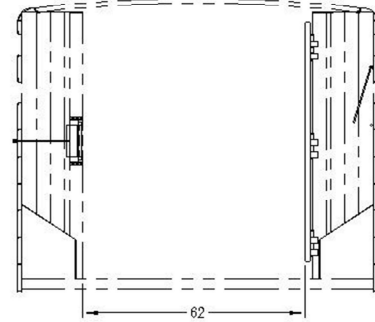
PASS-THROUGH WIDTH W/ 10K AXLES SHOWN WITH CENTER GATE OPEN
