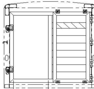
PASS-THROUGH WIDTH STANDARD SLIDING REAR GATE SHOWN WITH ROLLER GATE OPEN
