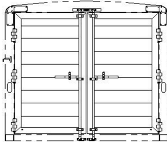
6'8" TALL, DOUBLE DOORS REAR OPENING - 88 7/8W X 75T CAM LATCH WITH STANDARD HINGES
