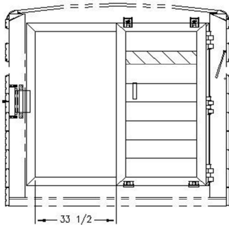
PASS-THROUGH WIDTH W/ 6K, 7K OR 7.2K AXLES SHOWN WITH ROLLER DOOR OPEN
