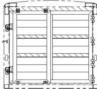
7'4" TALL, SLOTTED ROLLER GATE REAR OPENING - 82W X 84T
