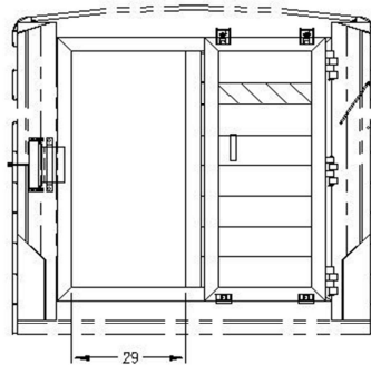
PASS-THROUGH WIDTH W/ 8K AXLES SHOWN WITH ROLLER DOOR OPEN
