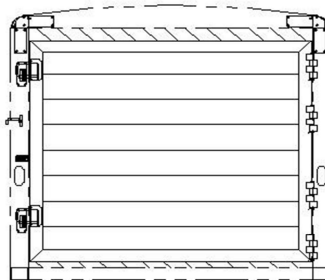
6'8" TALL, ENCLOSED SOLID GATE REAR OPENING - 82W X 76T
