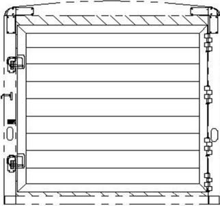
7'4" TALL, ENCLOSED SOLID GATE REAR OPENING - 82W X 84T
