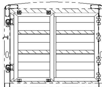
6'8" TALL, SLOTTED ROLLER GATE REAR OPENING - 82W X 76T
