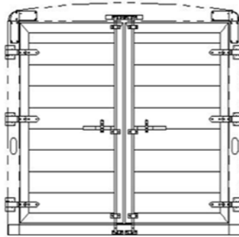
6'8" TALL DOUBLE DOOR REAR OPENING - 88 7/8" X 75" CAM LATCH WITH LAY-FLAT HINGES
