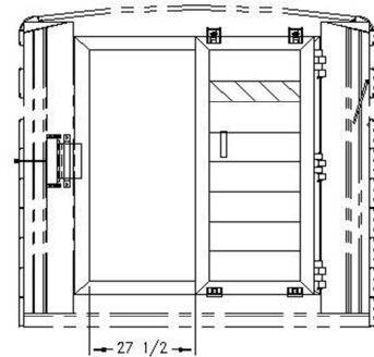
PASS-THROUGH WIDTH W/ 10K AXLES SHOWN WITH ROLLER DOOR OPEN
