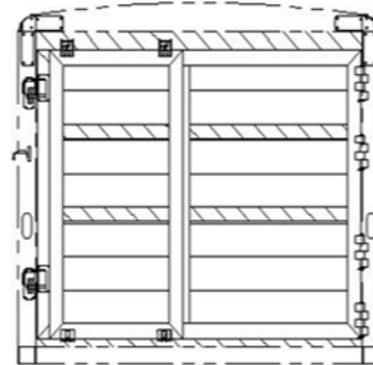
6'8" TALL, SLOTTED ROLLER GATE REAR OPENING - 90 1/2" X 76"
