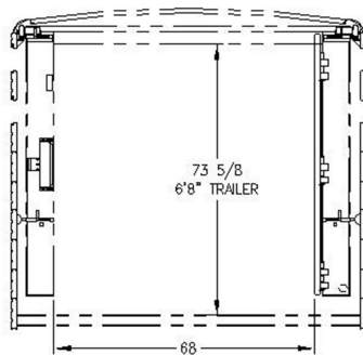
PASS-THROUGH DIMENSIONS ADJUSTABLE POSITION CENTER GATE
