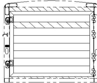
6'8" TALL, SOLID GATE REAR OPENING - 82W X 76T
