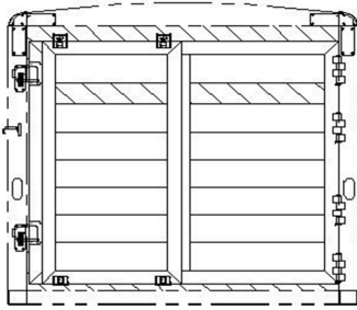
6'8" TALL, STANDARD LIVESTOCK SLIDER REAR OPENING - 82W X 76T
