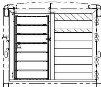
6'8" TALL, HALF ROLL-UP, 32 1/4" OPENING WIDTH REAR OPENING - 82W X 76T
