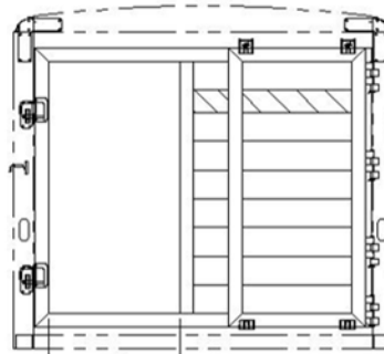
PASS-THROUGH WIDTH STANDARD SLIDING REAR GATE SHOWN WITH ROLLER GATE OPEN
