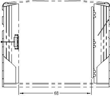
PASS-THROUGH WIDTH W/ 8K AXLES SHOWN WITH CENTER GATE OPEN
