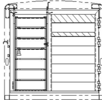
6'8" TALL, HALF ROLL-UP, 32 1/4" OPENING WIDTH REAR OPENING - 90 1/2" X 76"
