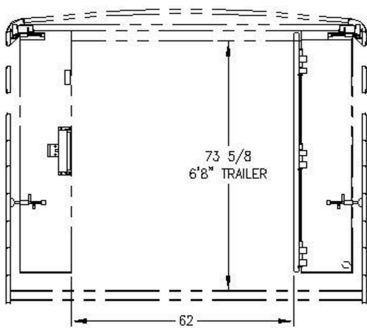
PASS-THROUGH DIMENSIONS ADJUSTABLE POSITION CENTER GATE
