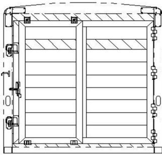
7'4" TALL, STANDARD LIVESTOCK SLIDER REAR OPENING - 82W X 84T
