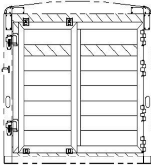
6'8" TALL, STANDARD LIVESTOCK SLIDER REAR OPENING - 82W X 76T
