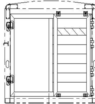
35 PASS-THROUGH WIDTH STANDARD SLIDING REAR GATE SHOWN WITH ROLLER GATE OPEN
