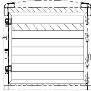
6'8" TALL, SOLID GATE REAR OPENING - 90 1/2" W X 76" T
