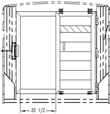
PASS-THROUGH WIDTH W/ 6K, 7K OR 7.2K AXLES SHOWN WITH CENTER GATE OPEN
