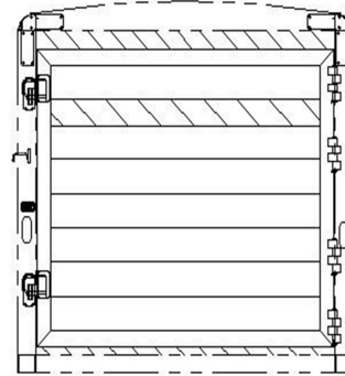
6'8" TALL, SOLID GATE REAR OPENING - 82W X 76T
