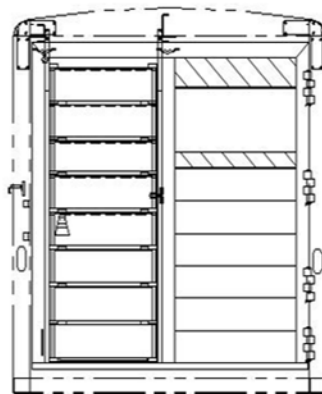
7'4" TALL, HALF ROLL-UP, 32 1/4" OPENING WIDTH REAR OPENING - 82W X 84T
