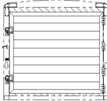
7'4" TALL, ENCLOSED SOLID GATE REAR OPENING - 90 1/2W X 84T
