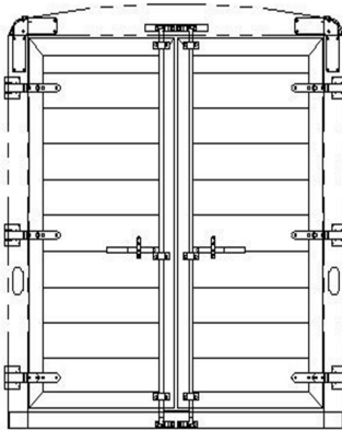
7'4" TALL, 7W, DOUBLE DOOR REAR OPENING - 74 3/8W X 83T CAM LATCH WITH LAY-FLAT HINGES
