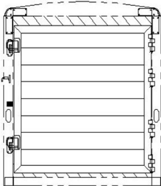
6'8" TALL, ENCLOSED SOLID GATE REAR OPENING - 76W X 76T
