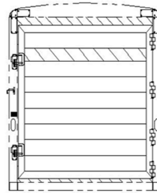
7'4" TALL, SOLID GATE REAR OPENING - 82W X 84T
