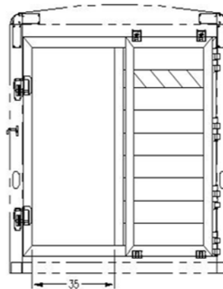
35 PASS-THROUGH WIDTH STANDARD SLIDING REAR GATE SHOWN WITH ROLLER GATE OPEN
