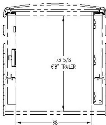
PASS-THROUGH DIMENSIONS ADJUSTABLE POSITION CENTER GATE
