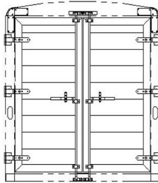
6'8" TALL, DOUBLE DOOR REAR OPENING - 74 3/8W X 75T CAM LATCH WITH LAY-FLAT HINGES
