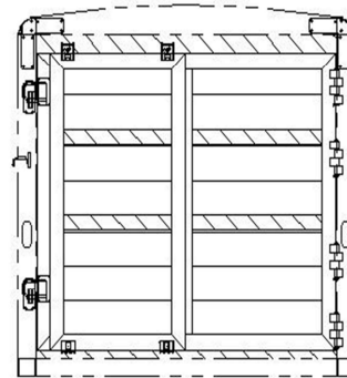
6'8" TALL, SLOTTED ROLLER GATE REAR OPENING - 82W X 76T
