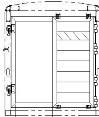
← 33 1/2 → PASS-THROUGH WIDTH STANDARD SLIDING REAR GATE SHOWN WITH ROLLER GATE OPEN
