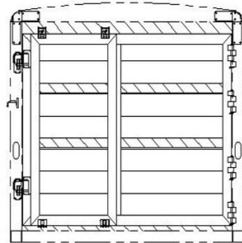
6'8" TALL, SLOTTED ROLLER GATE REAR OPENING - 90 1/2" W X 76" T
