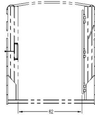
PASS-THROUGH WIDTH W/ 10K AXLES SHOWN WITH CENTER GATE OPEN
