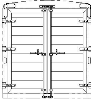
6'8" TALL, DOUBLE DOOR REAR OPENING - 88 7/8W X 75T CAM LATCH WITH LAY-FLAT HINGES
