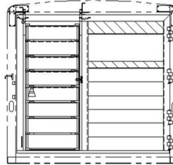
7'4" TALL, HALF ROLL-UP, 32 1/4" OPENING WIDTH REAR OPENING - 90 1/2W X 84T
