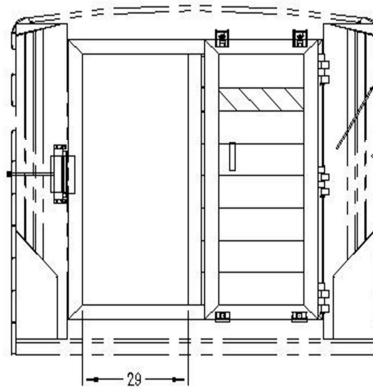
PASS-THROUGH WIDTH W/ 8K AXLES SHOWN WITH CENTER GATE OPEN
