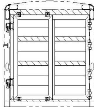
6'8" TALL, SLOTTED ROLLER GATE REAR OPENING - 76W X 76T
