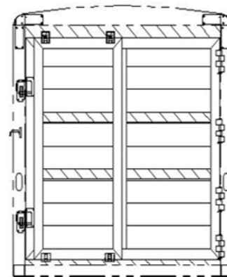
7'4" TALL, SLOTTED ROLLER GATE REAR OPENING - 82W X 84T
