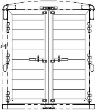
6'8" TALL, DOUBLE DOORS REAR OPENING - 74 3/8W X 75T CAM LATCH WITH STANDARD HINGES
