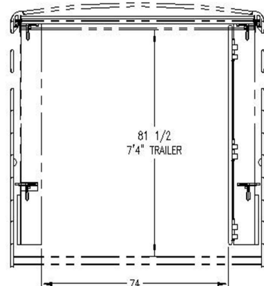
PASS-THROUGH DIMENSIONS ADJUSTABLE POSITION CENTER GATE
