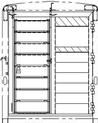
7'4" TALL, HALF ROLL-UP, 32 1/4" OPENING WIDTH REAR OPENING - 76W X 84T
