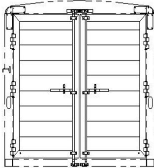
6'8" TALL, DOUBLE DOORS REAR OPENING - 88 7/8W X 75T CAM LATCH WITH STANDARD HINGES
