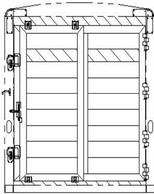
7'4" TALL, STANDARD LIVESTOCK SLIDER REAR OPENING - 76W X 84T
