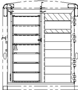
6'8" TALL, HALF ROLL-UP, 32 1/4" OPENING WIDTH REAR OPENING - 76W X 76T
