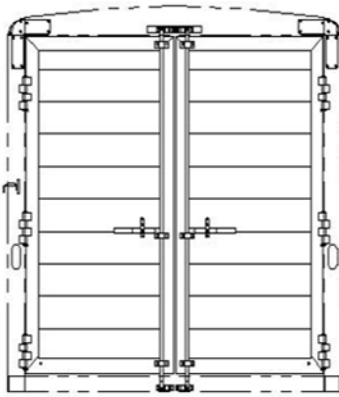
7'4" TALL, DOUBLE DOOR REAR OPENING - 88 7/8W X 83T CAM LATCH WITH STANDARD HINGES
