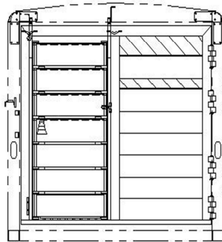
6'8" TALL, HALF ROLL-UP, 32 1/4" OPENING WIDTH REAR OPENING - 82W X 76T
