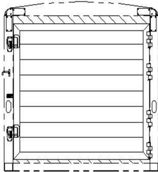
6'8" TALL, ENCLOSED SOLID GATE REAR OPENING - 82W X 76T
