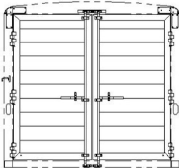
7'4" TALL, DOUBLE DOOR REAR OPENING - 88 7/8W X 83T CAM LATCH WITH STANDARD HINGES
