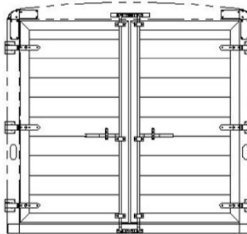
7'4" TALL, DOUBLE DOOR REAR OPENING - 88 7/8W X 83T CAM LATCH WITH LAT-FLAT HINGES
