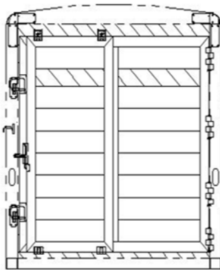
7'4" TALL, STANDARD LIVESTOCK SLIDER REAR OPENING - 82W X 84T
