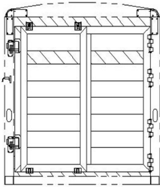
6'8" TALL, STANDARD LIVESTOCK SLIDER REAR OPENING - 76W X 76T
