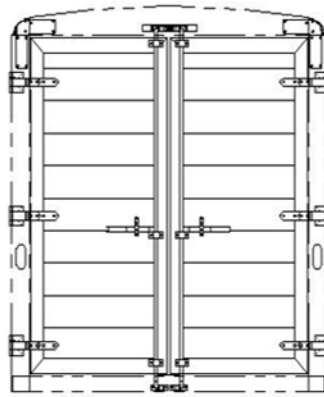
7'4" TALL, DOUBLE DOOR REAR OPENING - 88 7/8W X 83T CAM LATCH WITH LAY-FLAT HINGES
