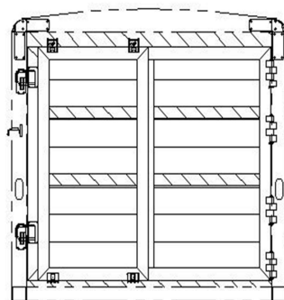
6'8" TALL, SLOTTED ROLLER GATE REAR OPENING - 82W X 76T
