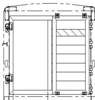
35 PASS-THROUGH WIDTH STANDARD SLIDING REAR GATE SHOWN WITH ROLLER GATE OPEN
