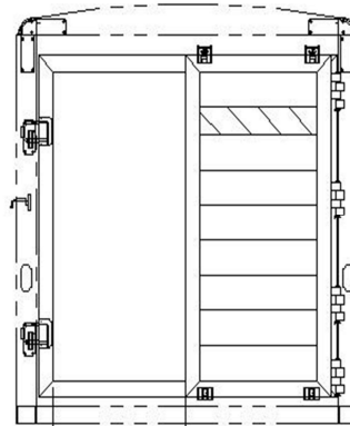
33 1/2" PASS-THROUGH WIDTH STANDARD SLIDING REAR GATE SHOWN WITH ROLLER GATE OPEN
