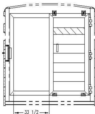
PASS-THROUGH WIDTH W/ 6K, 7K OR 7.2K AXLES SHOWN WITH ROLLER DOOR OPEN
