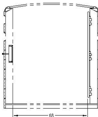
PASS-THROUGH WIDTH W/ 8K AXLES SHOWN WITH CENTER GATE OPEN
