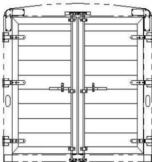
6'8" TALL, DOUBLE DOOR REAR OPENING - 88 7/8W X 75T CAM LATCH WITH LAY-FLAT HINGES
