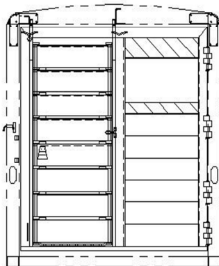
7'4" TALL, HALF ROLL-UP, 32 1/4" OPENING WIDTH REAR OPENING - 76W X 84T
