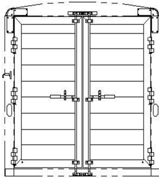
6'8" TALL, DOUBLE DOORS REAR OPENING - 74 3/8W X 75T CAM LATCH WITH STANDARD HINGES
