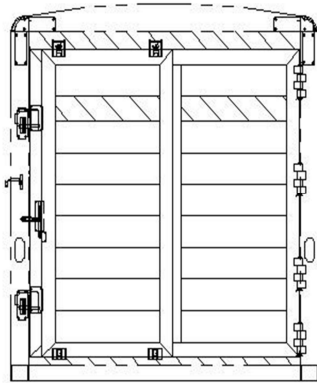
7'4" TALL, STANDARD LIVESTOCK SLIDER REAR OPENING - 76W X 84T
