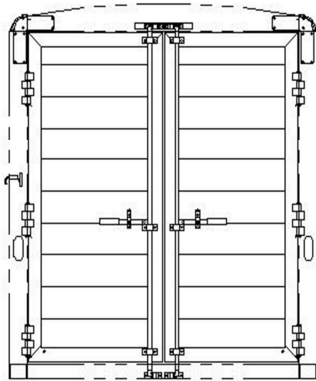
7'4" TALL, DOUBLE DOOR REAR OPENING - 74 3/8W X 83T CAM LATCH WITH STANDARD HINGES
