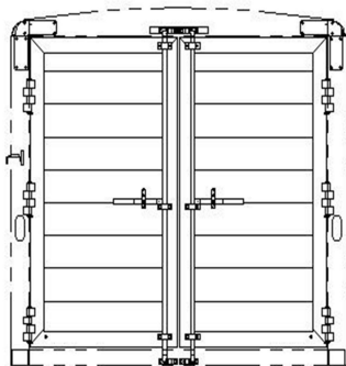
6'8" TALL, DOUBLE DOORS REAR OPENING - 88 7/8W X 75T CAM LATCH WITH STANDARD HINGES
