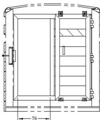
PASS-THROUGH WIDTH W/ 8K AXLES SHOWN WITH ROLLER DOOR OPEN
