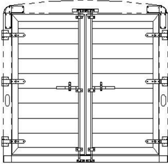
6'8" TALL, DOUBLE DOOR REAR OPENING - 88 7/8" W X 75" T CAM LATCH WITH LAY-FLAT HINGES
