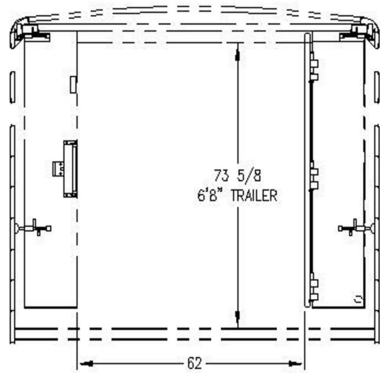
PASS-THROUGH DIMENSIONS ADJUSTABLE POSITION CENTER GATE
