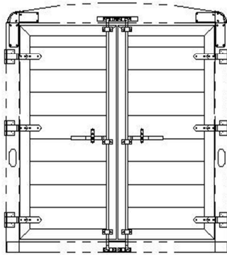
6'8" TALL, DOUBLE DOOR REAR OPENING - 74 3/8W X 75T CAM LATCH WITH LAY-FLAT HINGES
