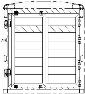
6'8" TALL, STANDARD LIVESTOCK SLIDER REAR OPENING - 76W X 76T
