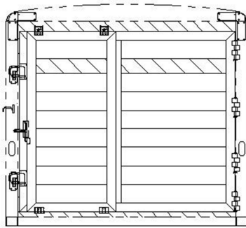
7'4" TALL, STANDARD LIVESTOCK SLIDER REAR OPENING - 90 1/2W X 84T
