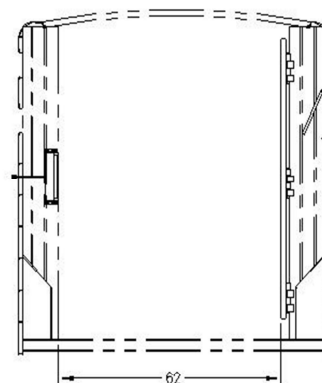
PASS-THROUGH WIDTH W/ 10K AXLES SHOWN WITH CENTER GATE OPEN
