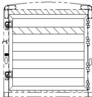
6'8" TALL, SOLID GATE REAR OPENING - 82W X 76T
