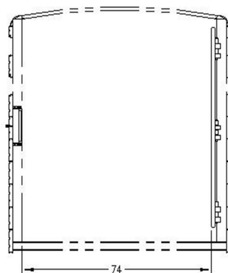
PASS-THROUGH WIDTH W/ 6K, 7K OR 7.2K AXLES SHOWN WITH CENTER GATE OPEN
