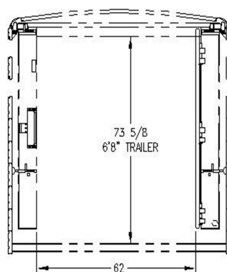
PASS-THROUGH DIMENSIONS ADJUSTABLE POSITION CENTER GATE
