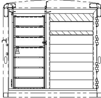
6'8" TALL, HALF ROLL-UP, 32 1/4" OPENING WIDTH REAR OPENING - 90 1/2" W X 76" T
