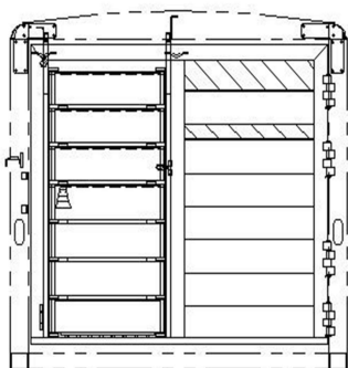
6'8" TALL, HALF ROLL-UP, 32 1/4" OPENING WIDTH REAR OPENING - 82W X 76T
