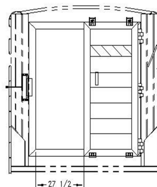
PASS-THROUGH WIDTH W/ 10K AXLES SHOWN WITH ROLLER DOOR OPEN
