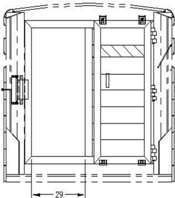
PASS-THROUGH WIDTH W/ 8K AXLES SHOWN WITH ROLLER DOOR OPEN
