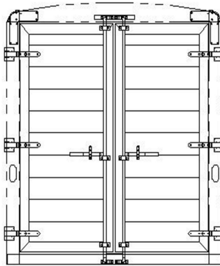
7'4" TALL, 7W, DOUBLE DOOR REAR OPENING - 74 3/8W X 83T CAM LATCH WITH LAY-FLAT HINGES
