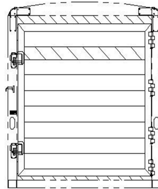
7'4" TALL, SOLID GATE REAR OPENING - 76W X 84T
