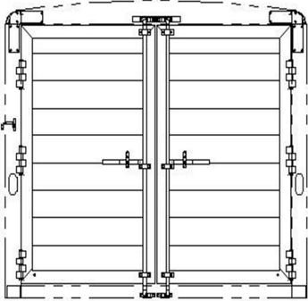
6'8" TALL, DOUBLE DOORS REAR OPENING - 88 7/8" W X 75" T CAM LATCH WITH STANDARD HINGES
