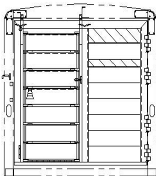
6'8" TALL, HALF ROLL-UP, 32 1/4" OPENING WIDTH REAR OPENING - 76W X 76T
