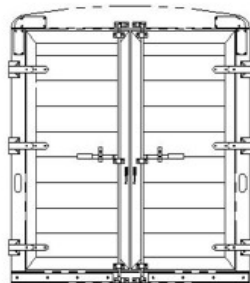
6'6" TALL, DOUBLE DOOR REAR OPENING - 74 3/8" X 72 1/2" CAM LATCH WITH LAY-FLAT HINGES
