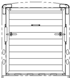
7'2" TALL, REAR RAMP REAR OPENING - 74 3/8" X 80 1/2"
