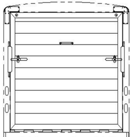
7'2" TALL, REAR RAMP REAR OPENING - 88 7/8" X 80 1/2"
