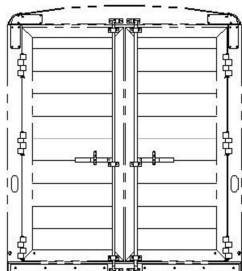
7'2" TALL, DOUBLE DOORS REAR OPENING - 74 3/8" X 80 1/2" CAM LATCH WITH STANDARD HINGES
