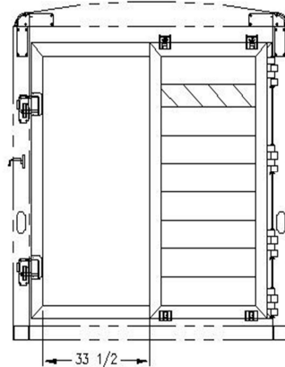
33 1/2 PASS-THROUGH WIDTH STANDARD SLIDING REAR GATE SHOWN WITH ROLLER GATE OPEN
