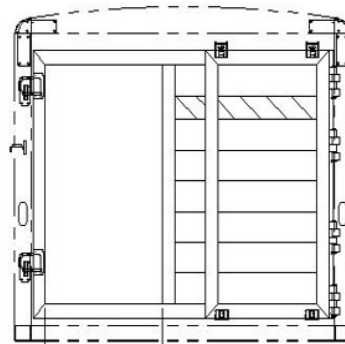
35" PASS-THROUGH WIDTH STANDARD SLIDING REAR GATE SHOWN WITH ROLLER GATE OPEN
