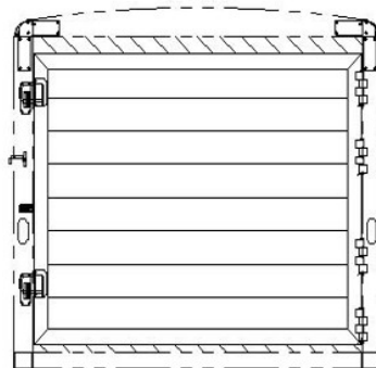
6'8" TALL, ENCLOSED SOLID GATE REAR OPENING - 90 1/2" W X 76" T
