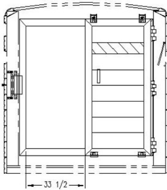
PASS-THROUGH WIDTH W/ 6K, 7K OR 7.2K AXLES SHOWN WITH ROLLER DOOR OPEN
