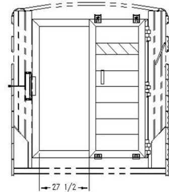
PASS-THROUGH WIDTH W/ 10K AXLES SHOWN WITH ROLLER DOOR OPEN
