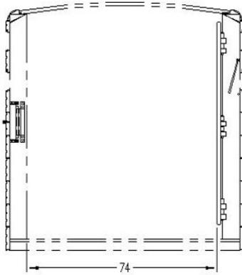
PASS-THROUGH WIDTH W/ 6K, 7K OR 7.2K AXLES SHOWN WITH CENTER GATE OPEN
