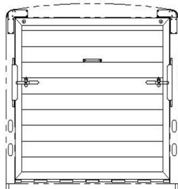
7'2" TALL, REAR RAMP REAR OPENING - 88 7/8" X 80 1/2"
