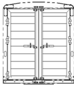
6'6" TALL, DOUBLE DOORS REAR OPENING - 74 3/8" X 72 1/2" CAM LATCH WITH STANDARD HINGES
