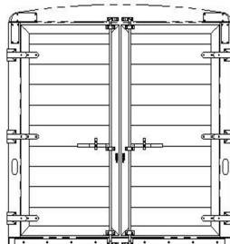
7'2" TALL, DOUBLE DOOR REAR OPENING - 88 7/8" X 80 1/2" CAM LATCH WITH LAY-FLAT HINGES
