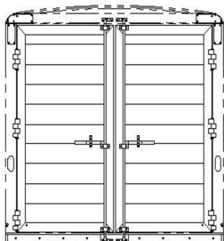
7'2" TALL, DOUBLE DOORS REAR OPENING - 88 7/8" X 80 1/2" CAM LATCH WITH STANDARD HINGES
