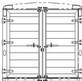
6'6" TALL, DOUBLE DOOR REAR OPENING - 88 7/8" X 72 1/2" CAM LATCH WITH LAY-FLAT HINGES
