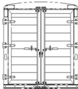
6'6" TALL, DOUBLE DOOR REAR OPENING - 74 3/8" X 72 1/2" CAM LATCH WITH LAY-FLAT HINGES
