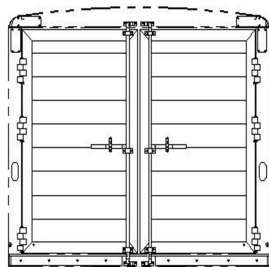
6'6" TALL, DOUBLE DOORS REAR OPENING - 88 7/8" X 72 1/2" CAM LATCH WITH STANDARD HINGES
