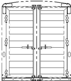
7'2" TALL, DOUBLE DOORS REAR OPENING - 74 3/8" X 80 1/2" CAM LATCH WITH STANDARD HINGES
