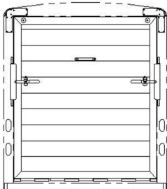
7'2" TALL, REAR RAMP REAR OPENING - 74 3/8" X 80 1/2"
