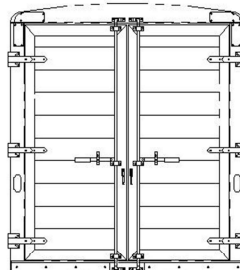
7'2" TALL, DOUBLE DOORS REAR OPENING - 74 3/8" X 80 1/2" CAM LATCH WITH LAY-FLAT HINGES
