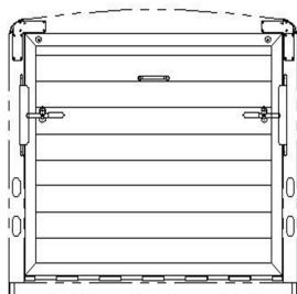
6'6" TALL, REAR RAMP REAR OPENING - 88 7/8" X 72 1/2"
